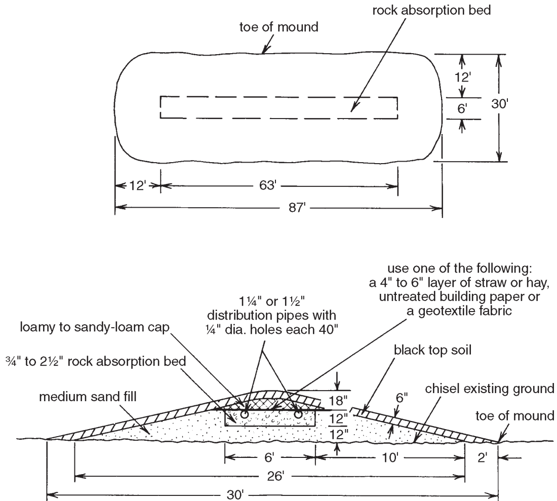
Figure 27. Sewage mound on flat terrain. The dimensions were calculated based on the effluent from a three-bedroom house with the mound built above a clay-loam to clay soil.
