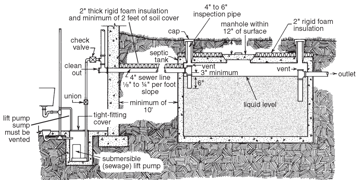
Figure 3. Shallow septic tank installation.
