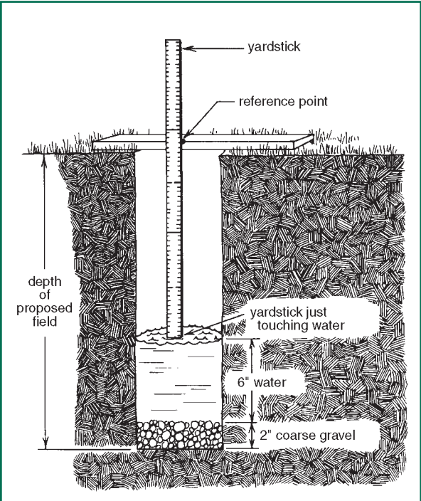
Figure 30. Soil percolation test hole and water level measuring apparatus.
